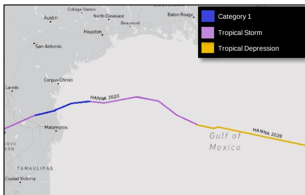
Track and intensity lifecycle of Hurricane Hanna. Image - NOAA, NHC
